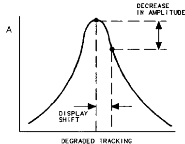
Figure 2-2. Tracking Error
