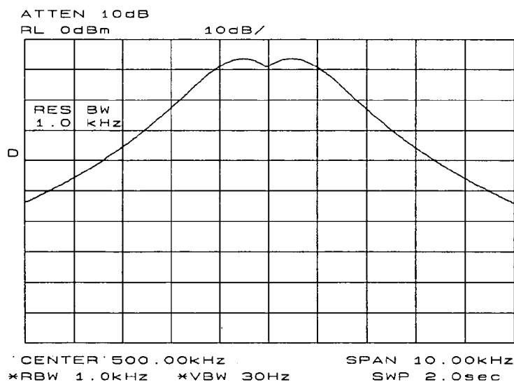
Figure G-1. 1 kHz Signal Separation
